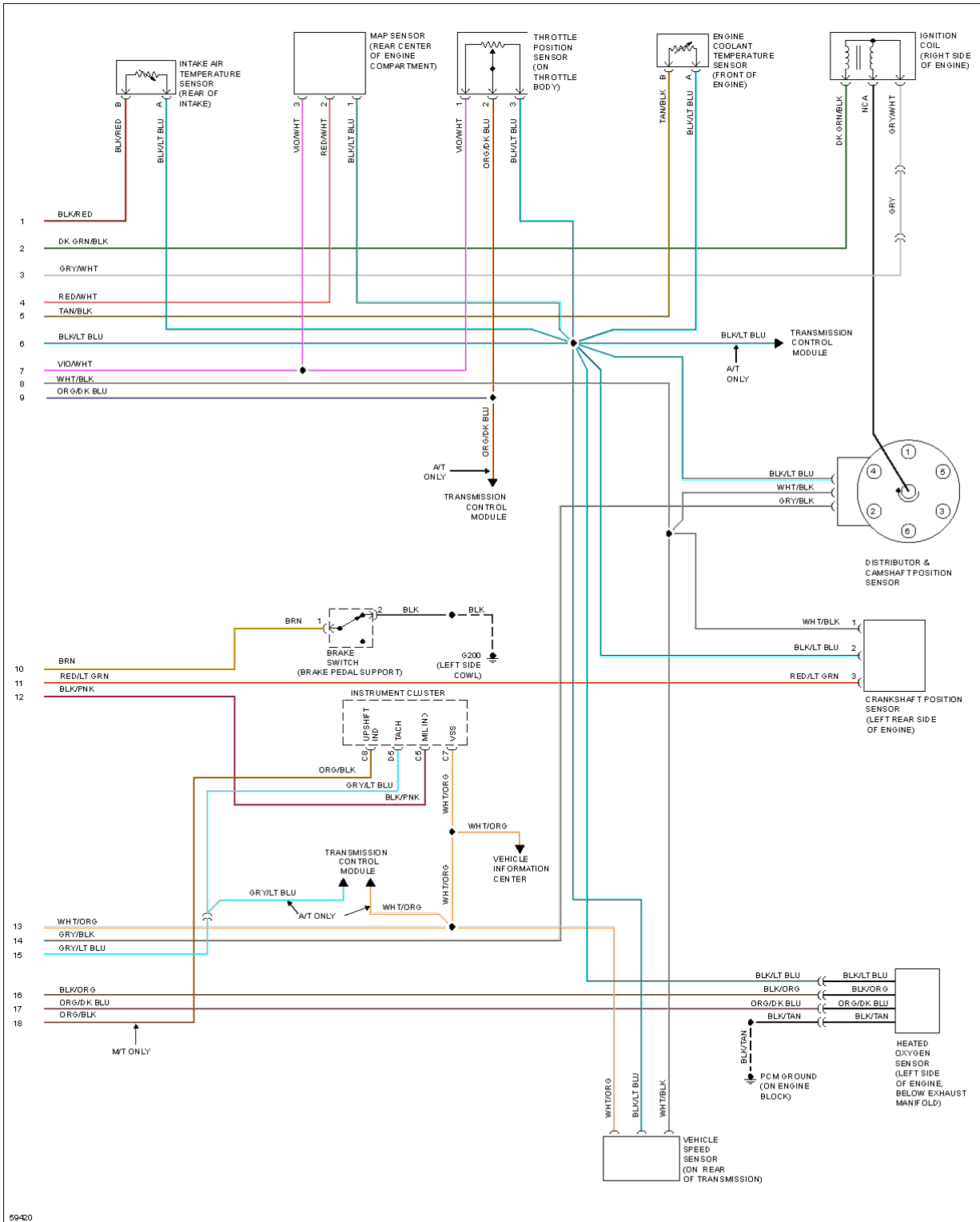
Fig. 7: 4.0L, Engine Performance Circuits (2 of 2)
