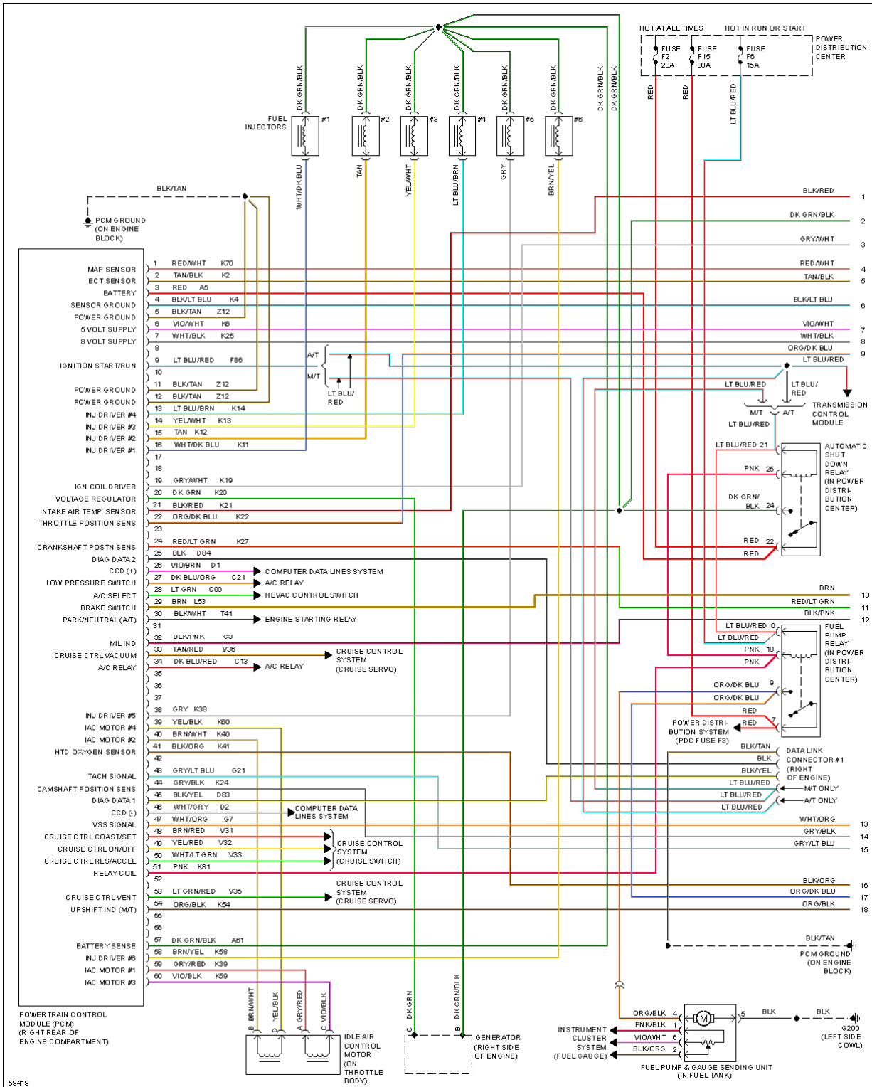
Fig. 6: 4.0L, Engine Performance Circuits (1 of 2)
